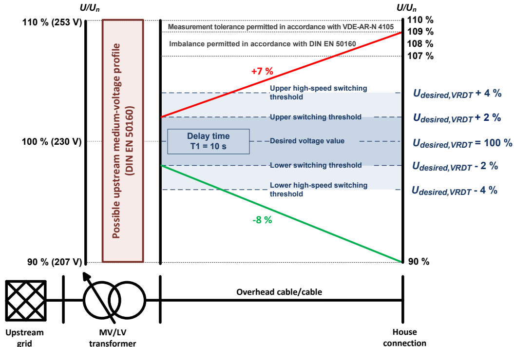
Figure 17: Voltage band distribution with VRDT at a desired voltage value of 100 % · U_n
