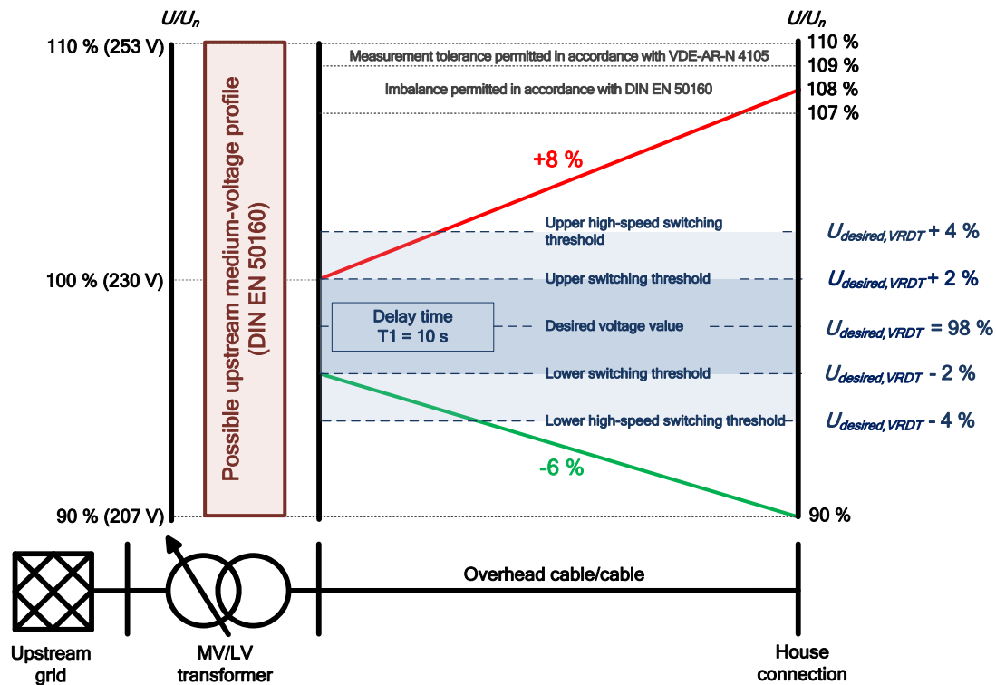
Figure 13: Example of distribution of the voltage band using VRDT at a desired voltage value of 98 % U_n (for explanations of delay time T_1 , see section 5.5.2)
