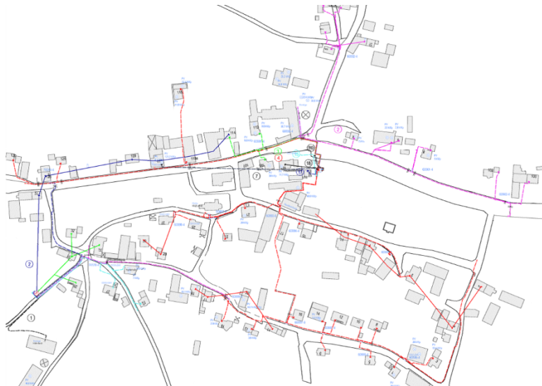
Figure 20: Grid section in accordance with example B3
