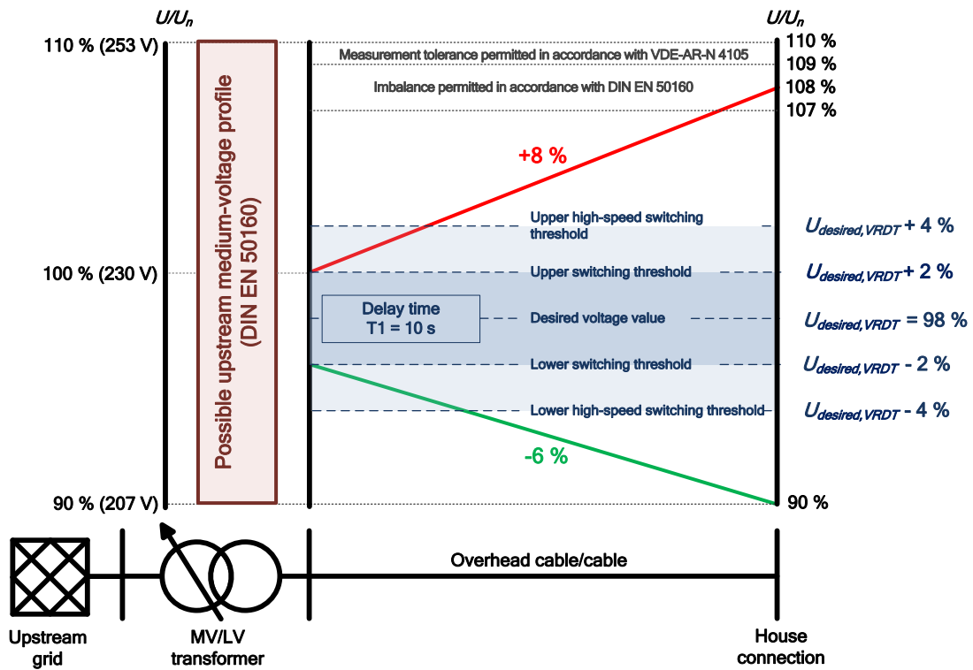
Figure 23: Example of voltage band distribution with VRDT at a desired voltage value of 98 % U_n
