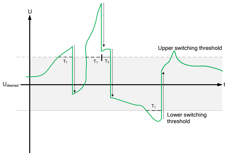
Figure 11: Use of a shortened delay time T_2
