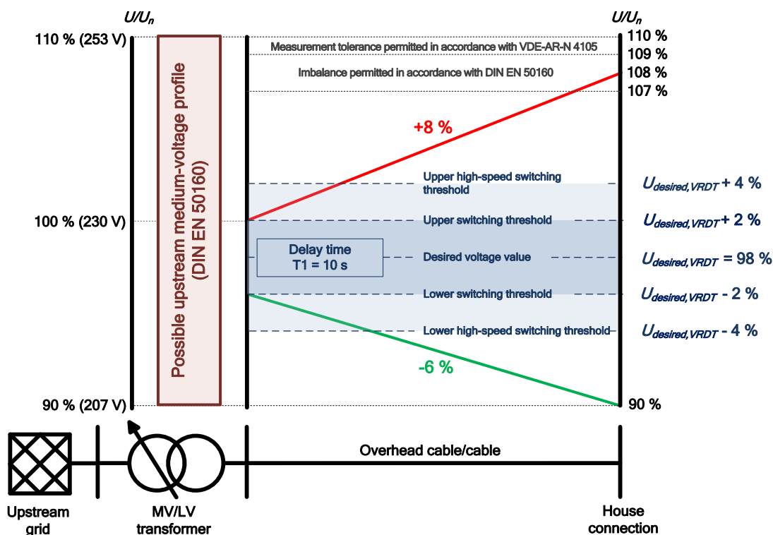
Figure 21: Example of voltage band distribution with VRDT at a desired voltage value of 98 % U_n
