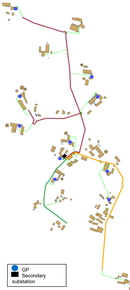
Figure 16: Grid section and description of a low-voltage grid in accordance with the example in B1
