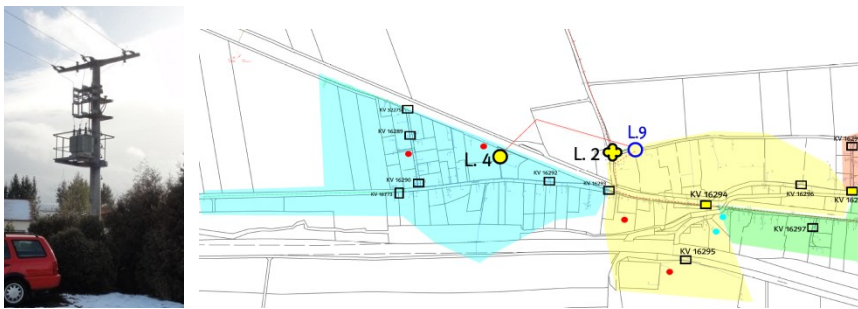
Figure 22: Grid section in accordance with example B4 -pole station and the two substation grids under consideration
